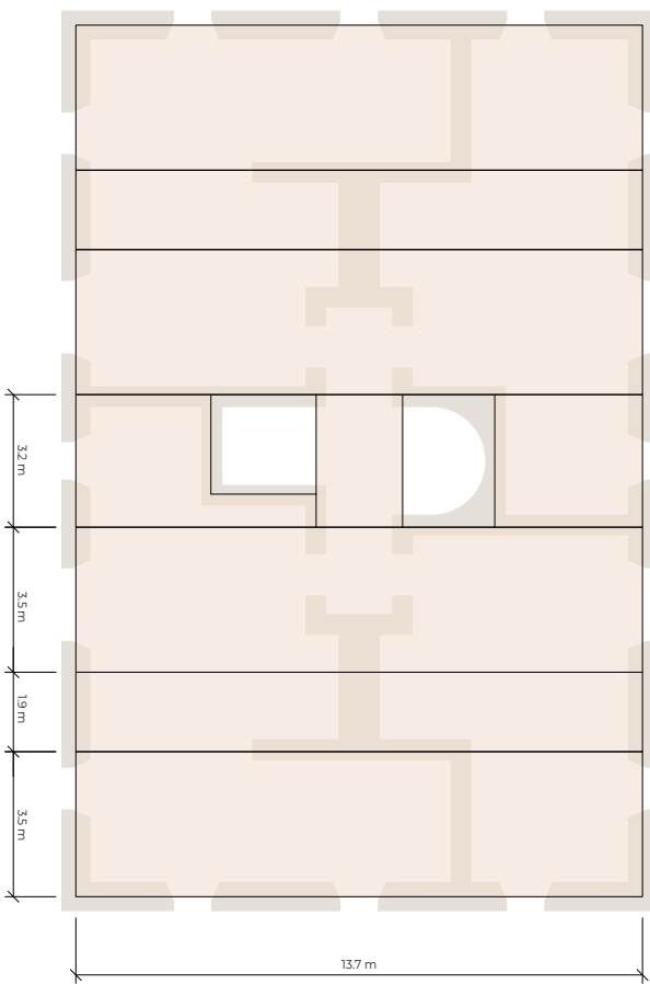
Figure 107. CLT slabs on top of the rammed earth walls.
