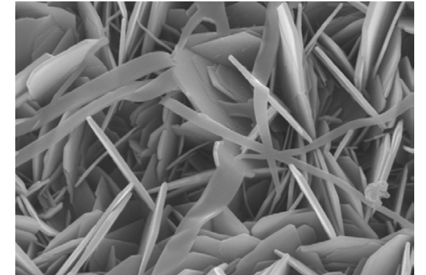
Figure 6. Clay particles are often formed as thin plates smaller than 2\text{ }\mu\text{m} , this gives clay its important cohesive property.
