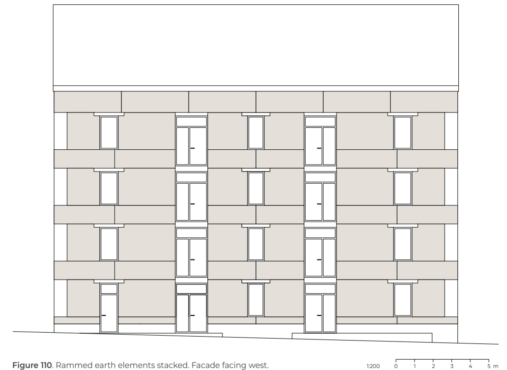
Figure 110. Rammed earth elements stacked. Facade facing west.
