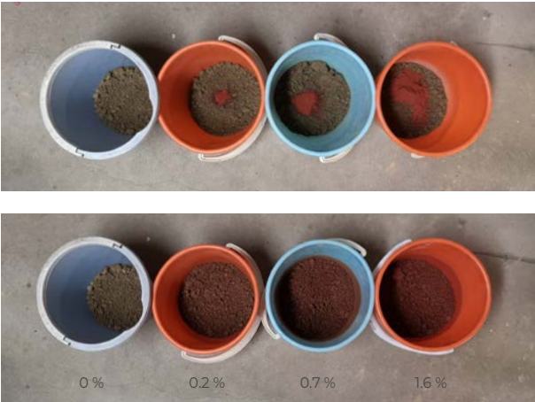
Figure 54. Pigmentation mixed with 2.5 kg of earth for each layer.
