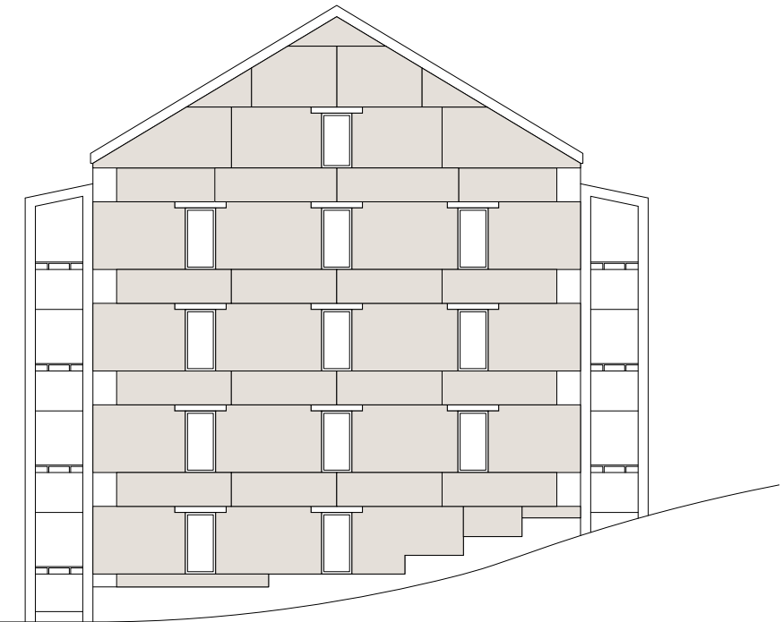
Figure 109. Rammed earth elements stacked. Facade facing south.
