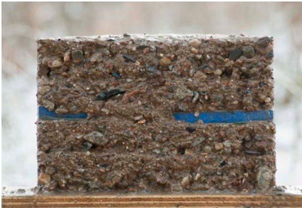
Figure 49. As the erosion progresses the erosion checks start to appear.
