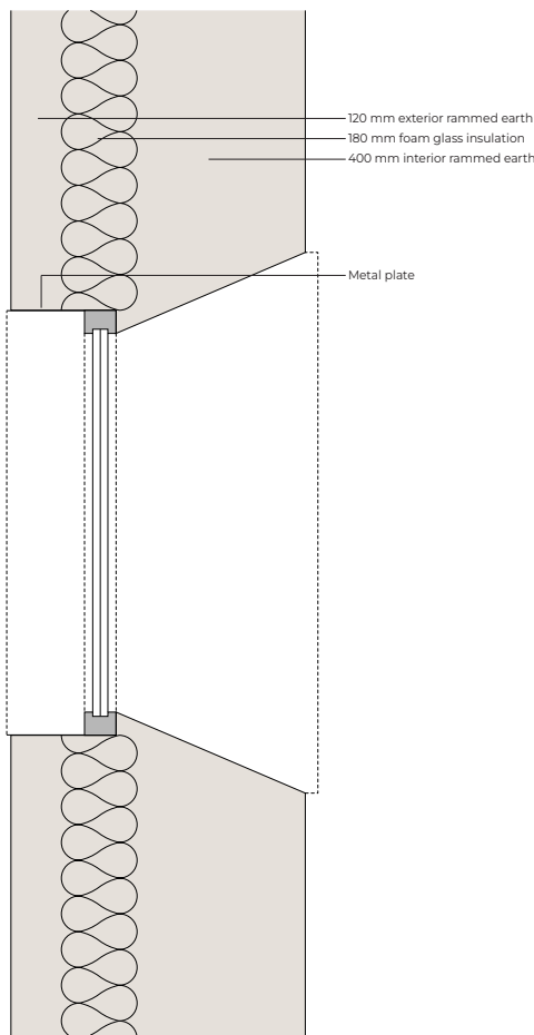
Figure 104. Window, top view.
