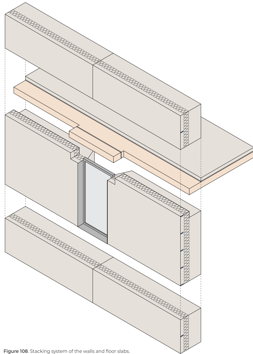
Figure 108. Stacking system of the walls and floor slabs.
