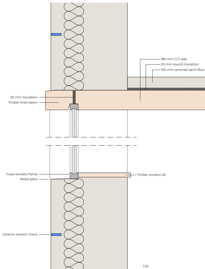
Figure 105. Window, side view.
