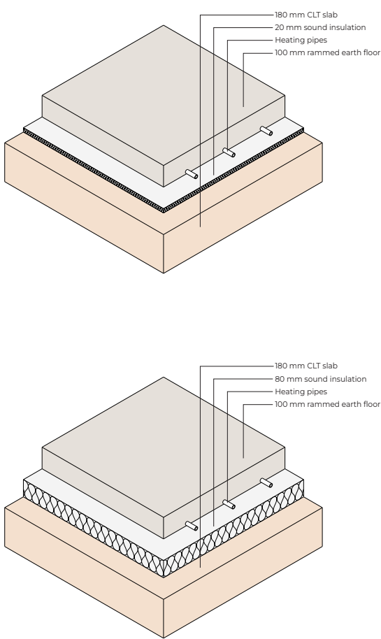
Figure 106. CLT and rammed earth floor construction details.
