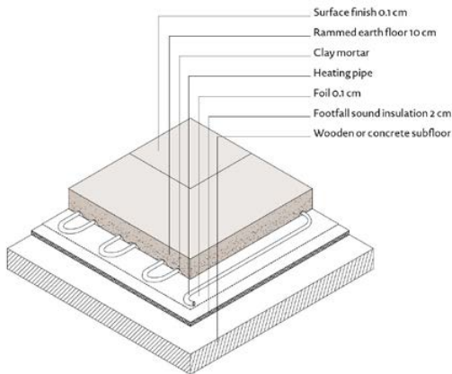
Figure 20. Rammed earth floor construction detail by Erden.
