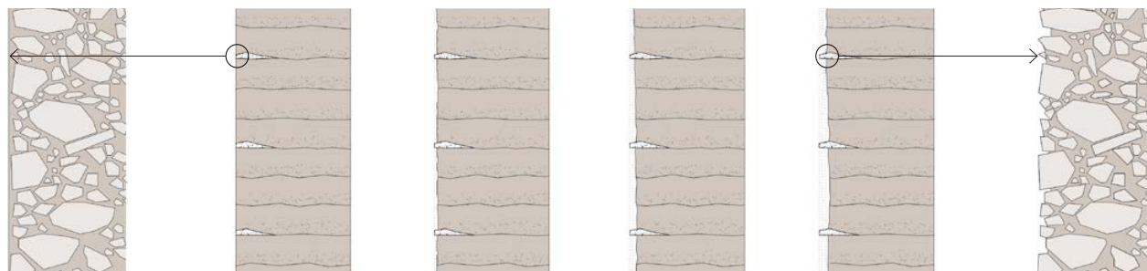
Figure 18. The rammed earth wall will erode between the erosion checks and get a rougher surface.
