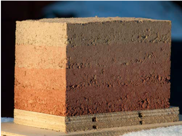
Figure 55. The pigmentation resulted in a nice gradiented rammed earth.
